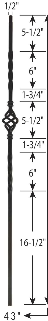
H-IB2552 Single Basket Double Twist
