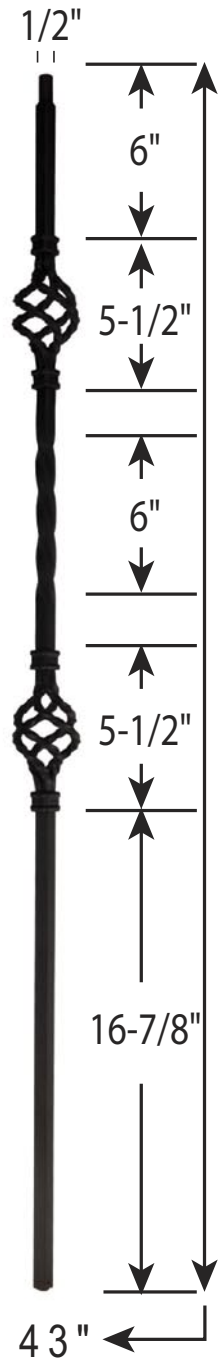
H-IB2553 Double Basket Single Twist
