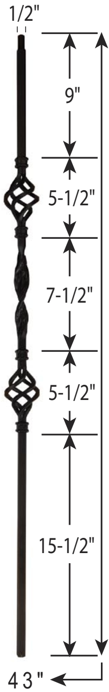
H-IB2565 Double Basket Single Ribbon
