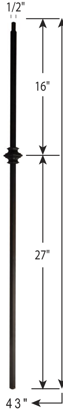
H-IB2550K Single Knuckle
