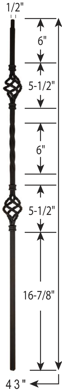
H-IB2557 Double Basket w/Twist Profile
