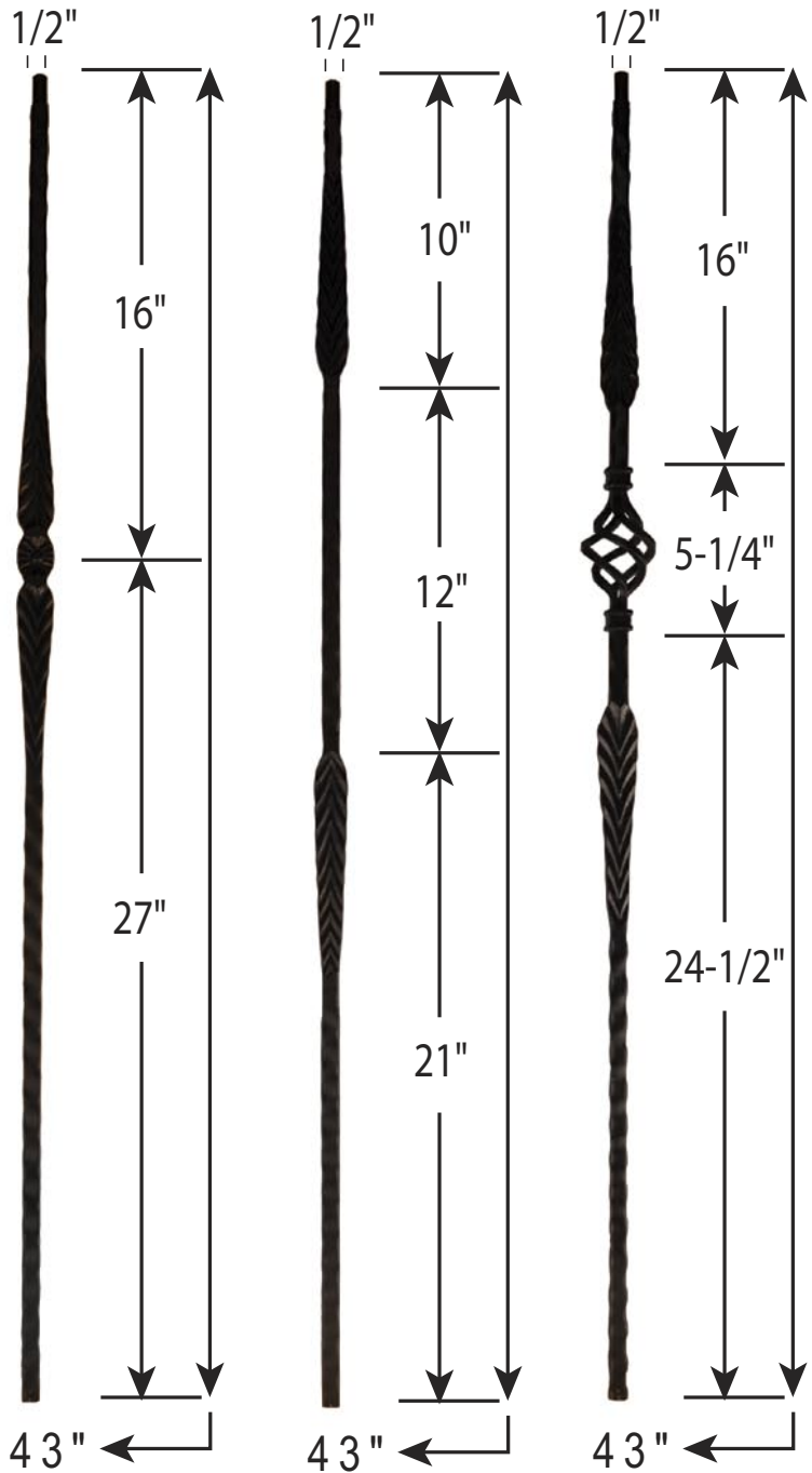
H-IB2510 Single Feather
