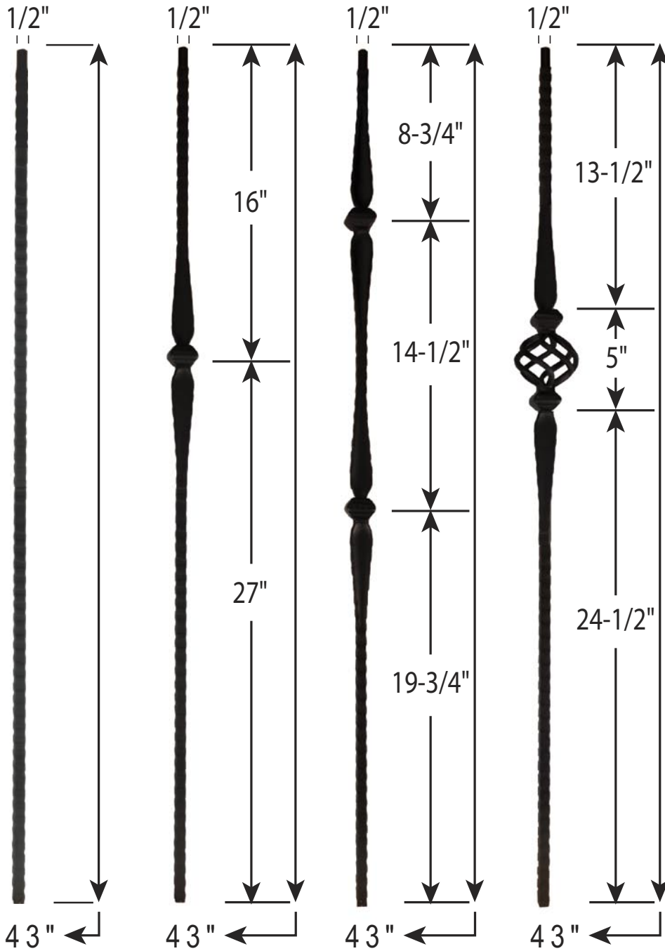
H-IB2517HE Gothic Plain Bar
