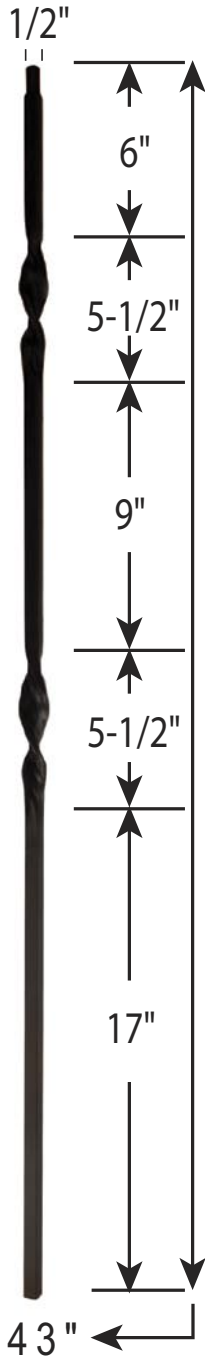
H-IB2561 Double Ribbon
