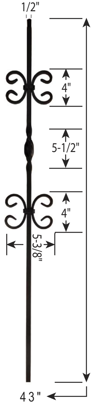
H-IB2563 Double Butterfly
