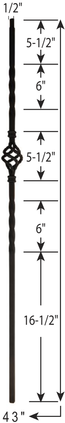
H-IB2556 Single Basket w/Twist Profile
